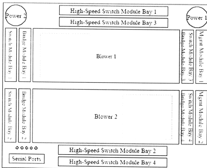
Figure 2. BladeCenter H (8852) rear view
