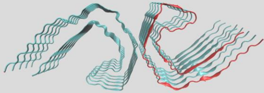
Amyloid protein
