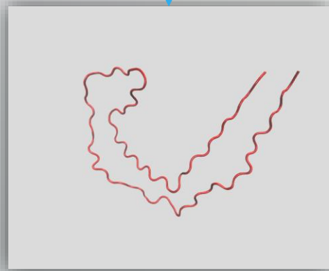
I-TASSER result
