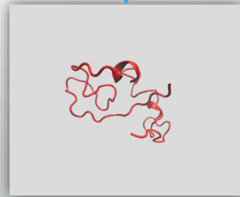
ROBETTA result
